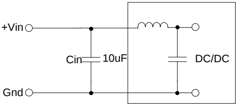
Input With External Capacitor
